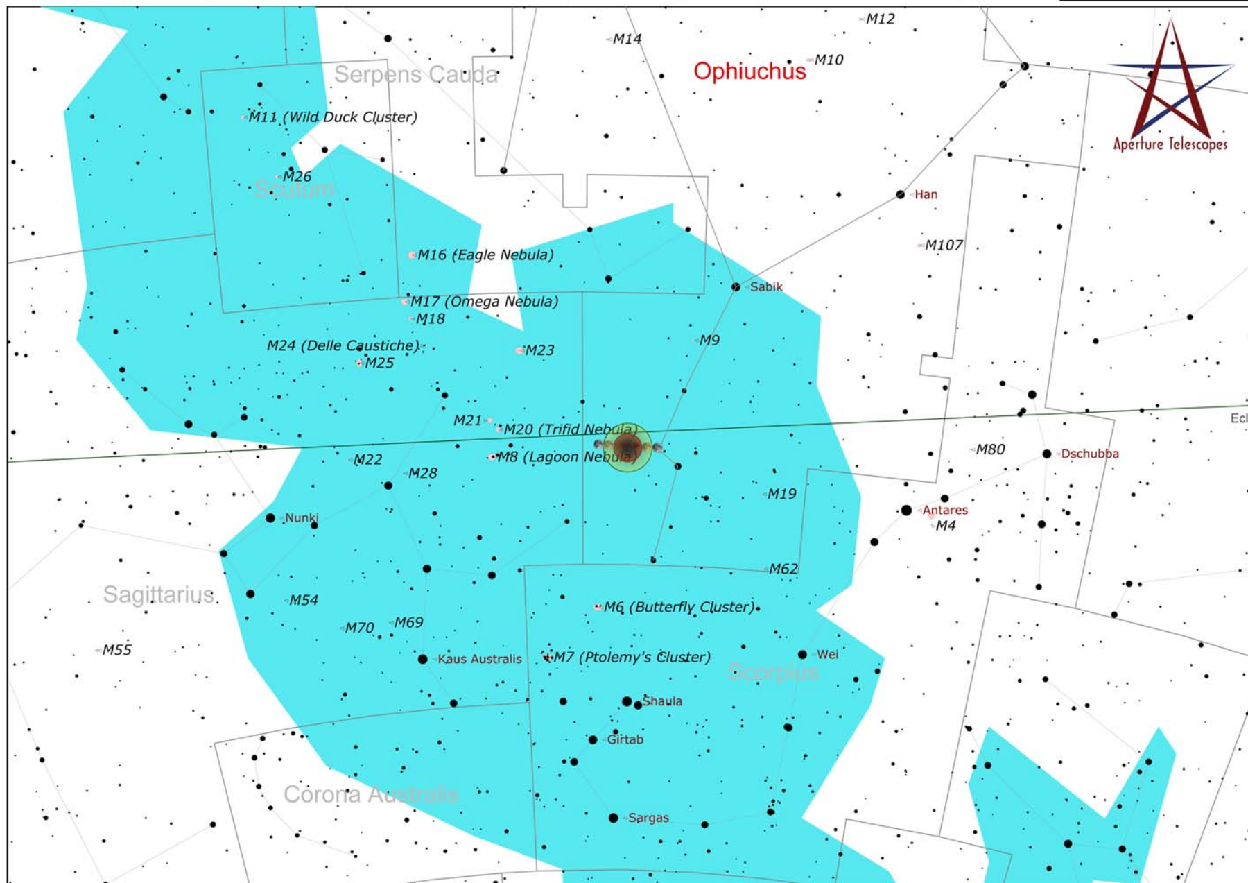
Sky Map showing the circumstances of Total Lunar Eclipse over Majkhali, Uttarakhand, India © Ajay Talwar F.O.V. ~60°
